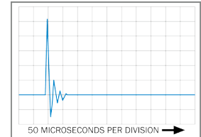
Impulse Response
