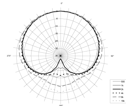
Fig. 4. Polar Response (Typical) of P30/C
