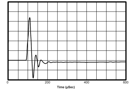
Fig. 3. Impulse Response (Typical) of P30/C
